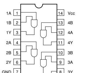
IC505: SN74LV08APWR Quadruple 2-input positive-AND gate
